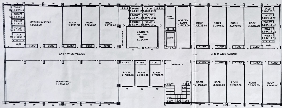
HOSTEL THIRD FLOOR PLAN-HATTA
